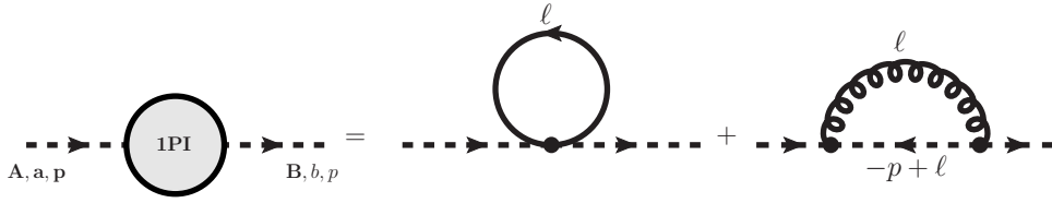
Figure 21. Diagrams for fermionic propagator at one-loop.
