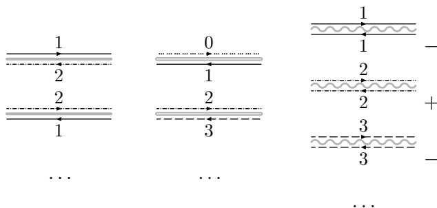
Figure 15. Double line notation for untwisted, twisted and gluon color lines, cf. figure 4. Gluon lines have associated sign factors.
