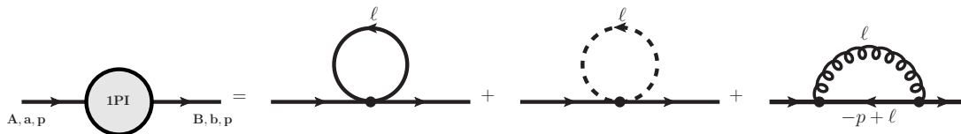
Figure 22. Diagrams for bosonic propagator at one-loop.
