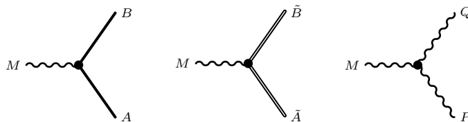
Figure 5. Color vertices: M_{MAB} , \tilde{M}_{M\bar{A}\bar{B}} , F_{MPQ} .
