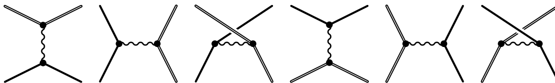
Figure 8. Mixed tree graphs: \Upsilon_{12,\bar{3}\bar{4}}^{(0)} , \Upsilon_{12,\bar{3}\bar{4}}^{(0)} , \Upsilon_{13,\bar{2}\bar{4}}^{(0)} , \Upsilon_{\bar{1}\bar{2},34}^{(0)} , \Upsilon_{\bar{1}\bar{2},34}^{(0)} , \Upsilon_{\bar{1}\bar{3},24}^{(0)} .
