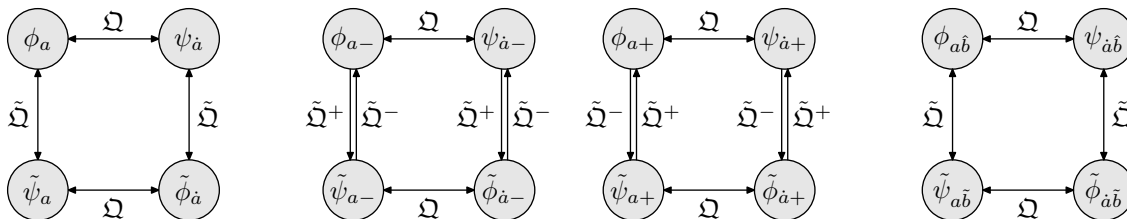
Figure 2. The action of the extended \mathcal{N} = 5, 6, 8 supersymmetries (left, middle two, right) on one-particle asymptotic states.
