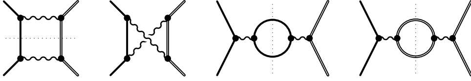
Figure 13. Mixed scattering at one loop with untwisted particles 1, 4 and twisted particles 2, 3: \mathcal{Y}_{14, \tilde{2}\tilde{3}}^{(1)\square} , \mathcal{Y}_{14, \tilde{3}\tilde{2}}^{(1)\square} , \mathcal{Y}_{14, \tilde{2}\tilde{3}}^{(1)\circ} , \mathcal{Y}_{14, \tilde{3}\tilde{2}}^{(1)\circ} .
