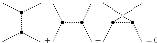
Figure 6. Jacobi identities for color structures.
