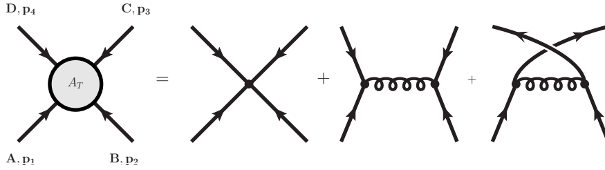
Figure 19. Diagrams for the A element at tree level.
