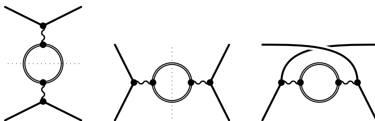
Figure 12. Untwisted scattering with internal twisted loop: \Upsilon_{12,34}^{(1)\circ} , \Upsilon_{14,23}^{(1)\circ} , \Upsilon_{13,24}^{(1)\circ} . The horizontal and vertical dotted lines indicate possible unitarity cuts in the s - and t -channels, respectively, to be discussed in section 6.5.
