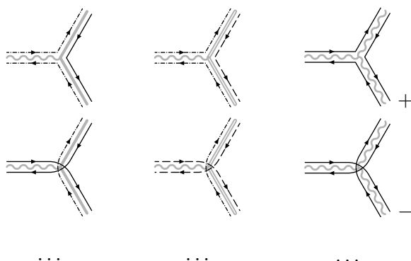
Figure 16. Double line notation for vertices, cf. figure 5. Pure gluon vertices have associated sign factors.
